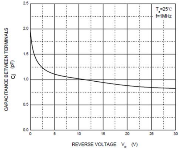
Fig 2: Capacitance Capability
