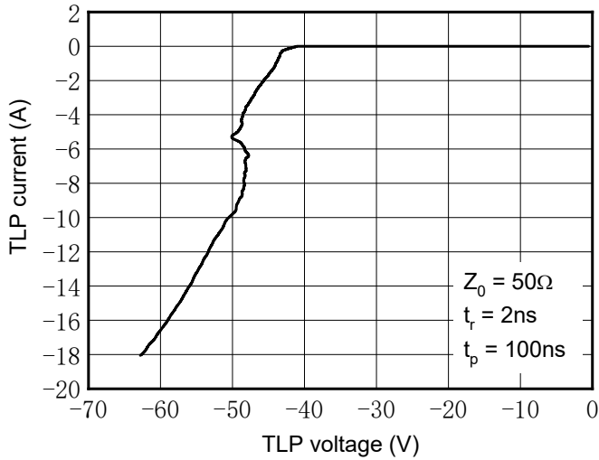
Fig.7 TLP Measurement
